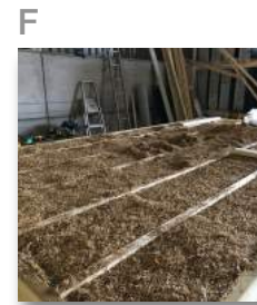
F Straw is installed into panel
