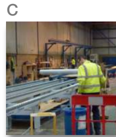
C Panel frames are assembled in a flying factory.
